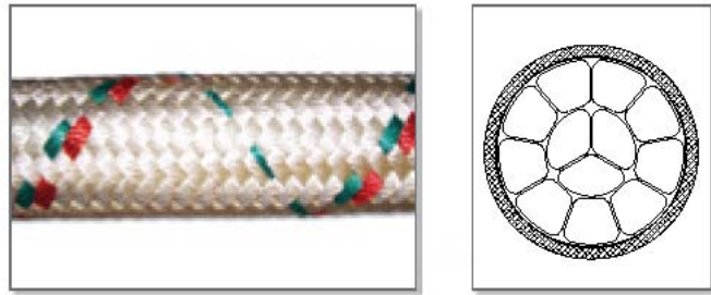
Rope in which components are laid parallel to each other within an outer braided jacket (also circular braided). The jacket is non-load bearing
